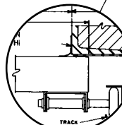
Top view of Jamb Seal
